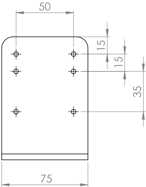
VIEW RELATIVE TO FRONT FACE
