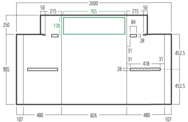
Graphic Size for Unit and Window Allow 37.5mm for top and bottom
